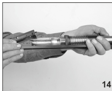
14. Pull back and remove the mechanism
